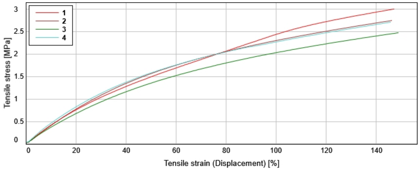
Specimen 1 to 4
